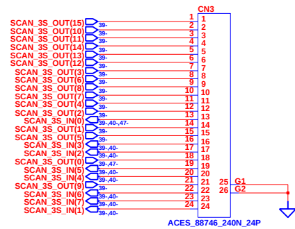
KEYBOARD CONN
